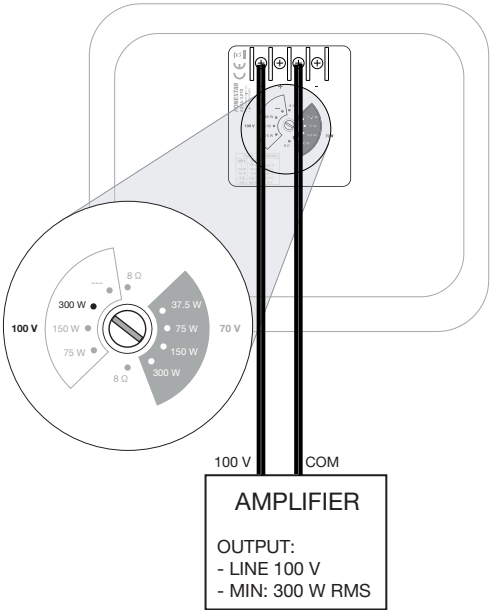
100 V LINE
